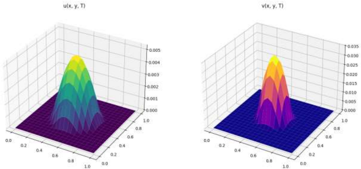
Figure 1 shows the numerical solution of problem (1) - (3). q_1 = 4.75, q_2 = 5.5, m_1 = 1.15, m_2 = 1.35
