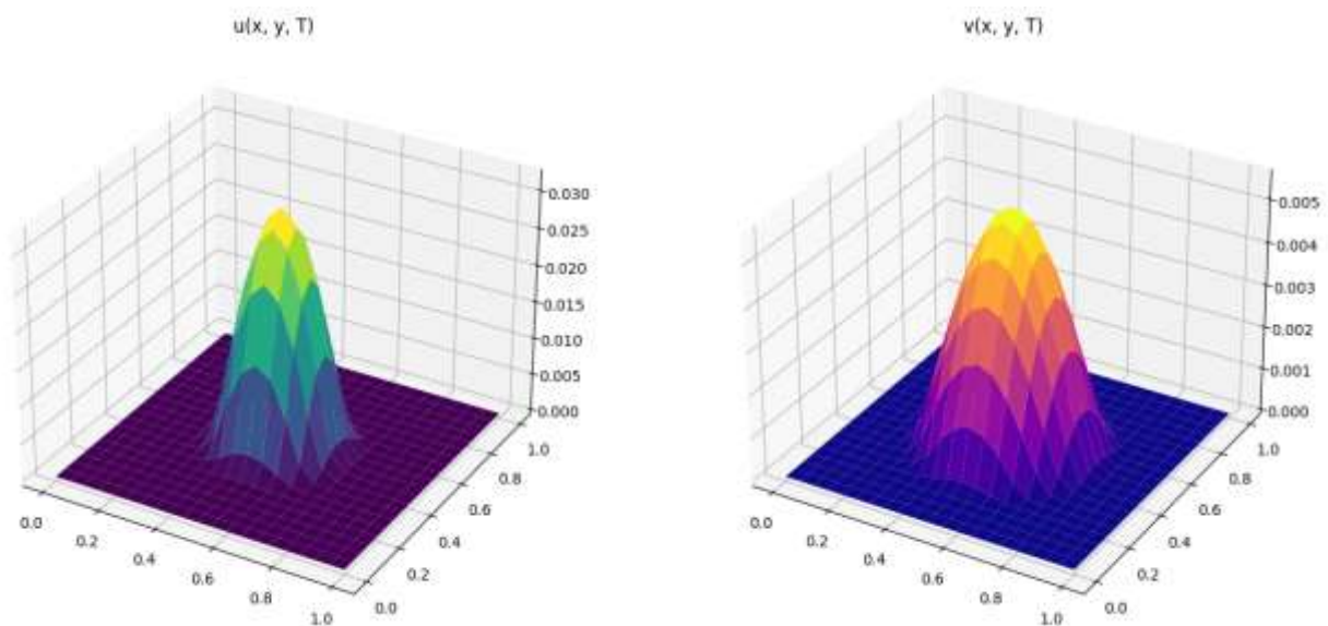
Figure 2 shows the numerical solution of problem (1) - (3). q_1 = 1.75, q_2 = 1.95, m_1 = 1.55, m_2 = 1.65
