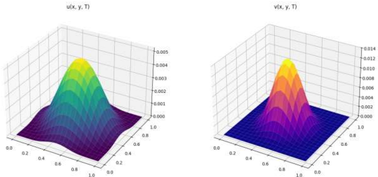
Figure 1 shows the numerical solution of problem (1) - (3). q_1 = 1.8 , q_2 = 2.3 , m_1 = 1.75 , m_2 = 1.25
